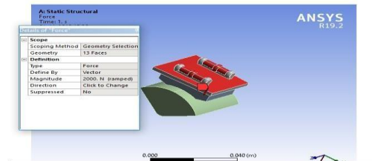
Fig 9 Meshing of ankle joint
