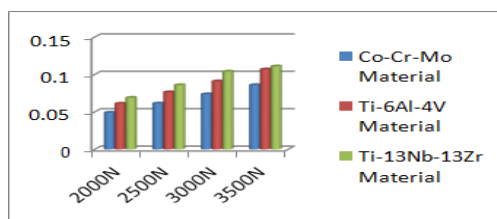
Graph.2 Total Deformation (mm)
