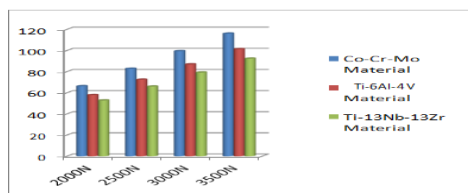
Graph.1 Von-mises stress (Mpa)
