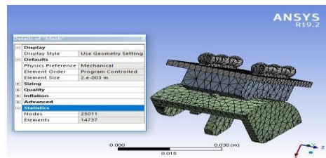
Fig.7 Design of Talar bearing
